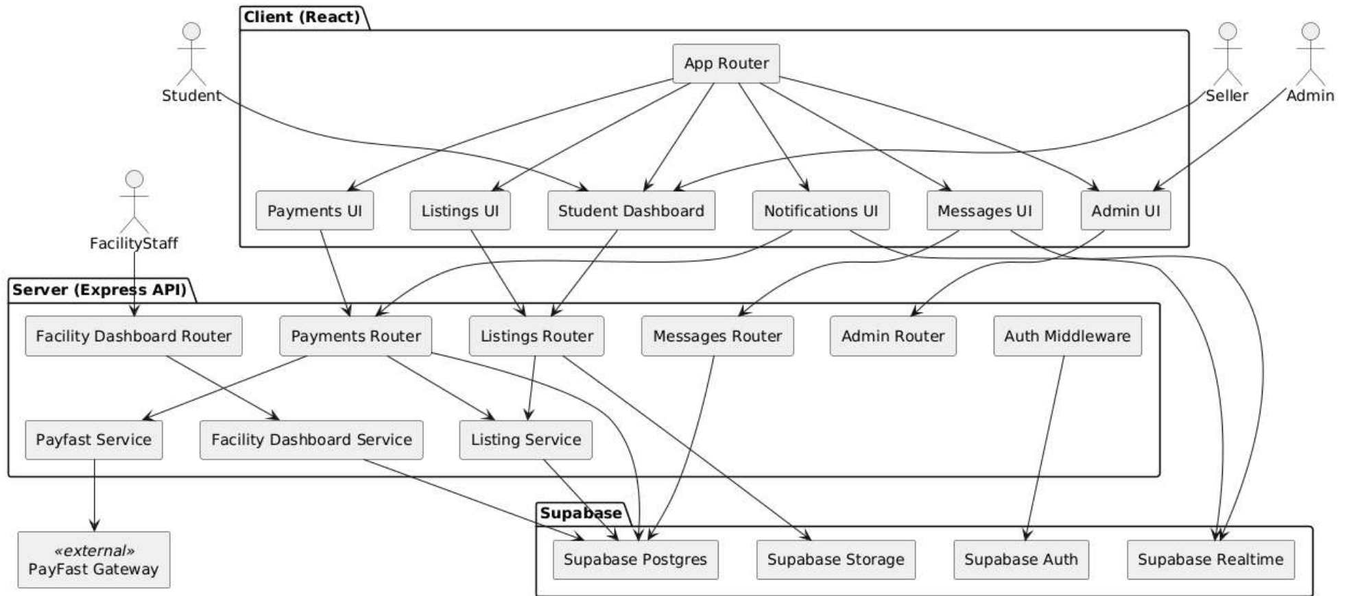
Component Diagram - Marketplace + Payments
